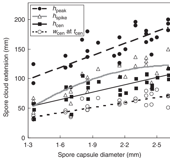
FIG. 4. Sphagnum spore cloud extensions after discharge in relation to capsule diameter: closed circles and long-dashed line (regression line) represent observations on peak height ( h_{peak} ) of the spore cloud; open triangles and grey curved line represent height of the spike ( h_{spike} ) just after discharge; closed squares and unbroken line represent height of the centroid (the average spore maximum; h_{cen} ); open circles and short-dashed line represent horizontal width of the spore cloud ( w_{cen} ) at the moment of centroid maximum ( t_{cen} ). The lines are based on the simple models in Table 2, except for h_{spike} that also includes the quadratic relationship to capsule diameter (the only term that showed improved adjusted R^2 when including the quadratic directly after the linear relationship).
